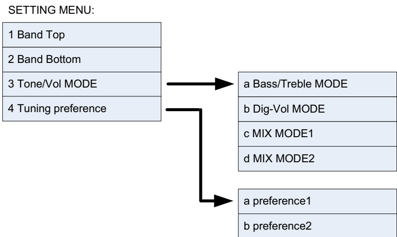
Figure 4. Setting Menu
